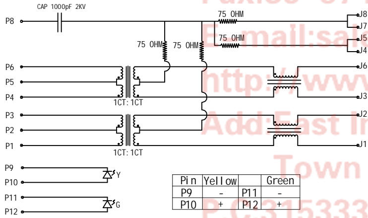
CIRCUIT SCHEMATIC
