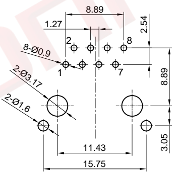
PCB layout Thickness=1.6mm
