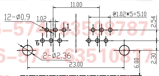
PC BOARD LAYOUT THICKNESS=1.6MM
