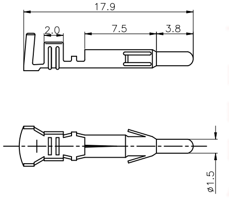
Male TERMINAL (For Female Housing)
