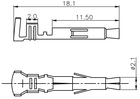
Male TERMINAL (For Female Housing)
