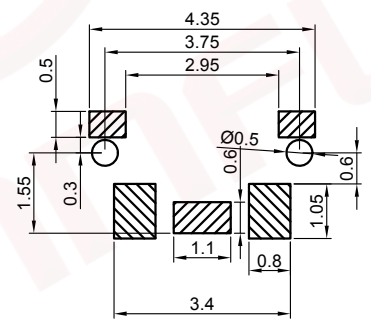
PCB layout Tolerance±0.05
